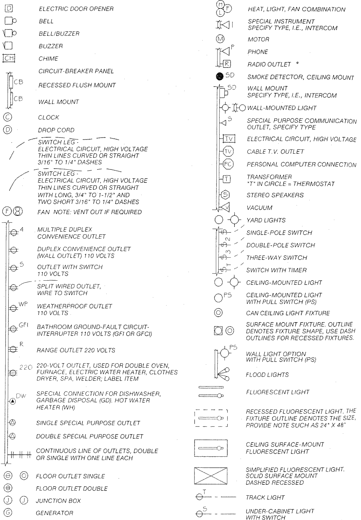
FIGURE 17.2 ■ Common electrical symbols.
